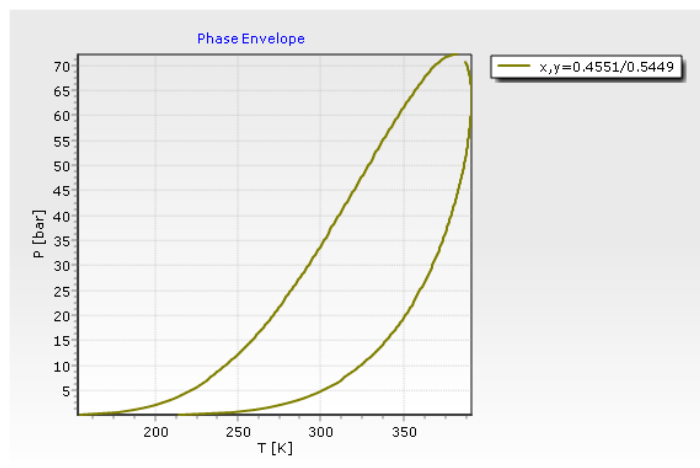
Phase Envelope Calculation with VTPR; Carbon dioxide and n-Butane
