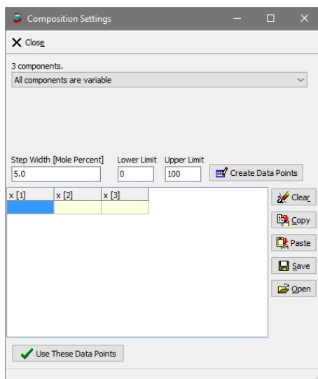
Figure 8: Composition settings
