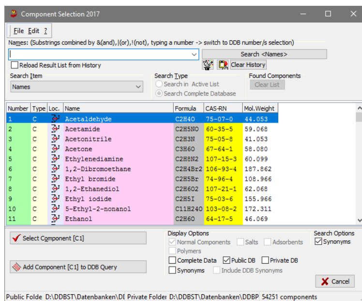
Figure 2: Component selection
